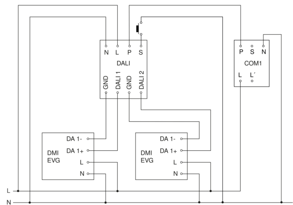
Master/master interconnection circuit diagram
